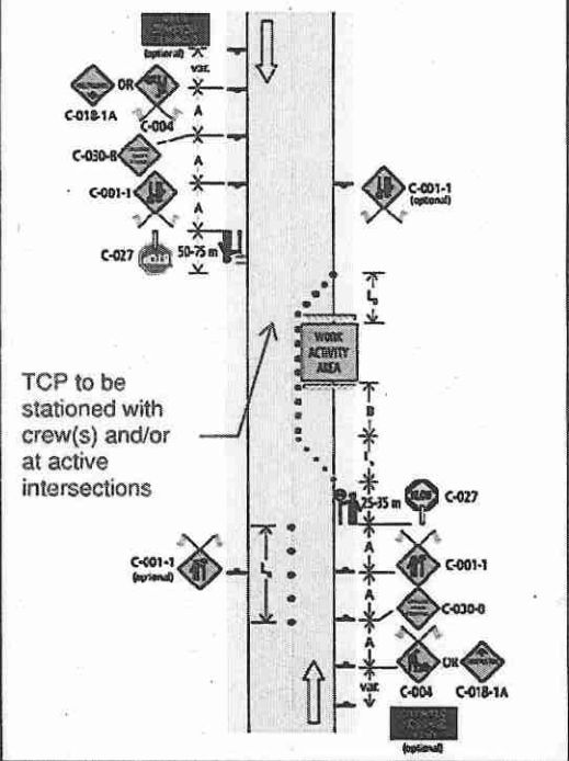
Figure 7.2: Lane Closure with TCPs – Single Lane Alternating – Short and Long Duration
